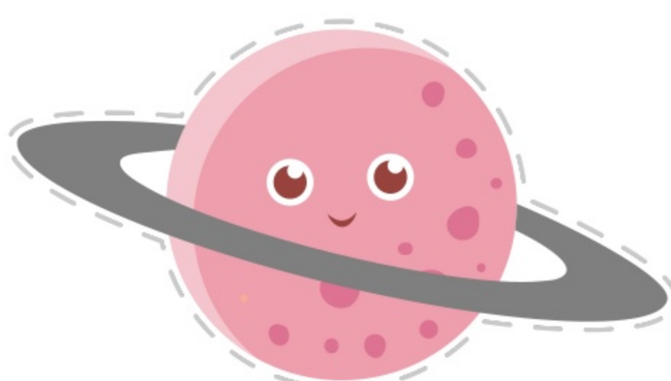
SATURN
