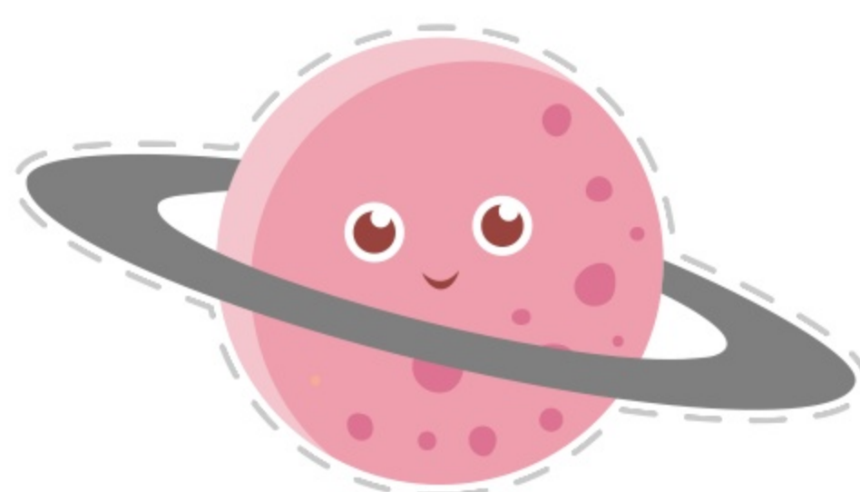
SATURN
