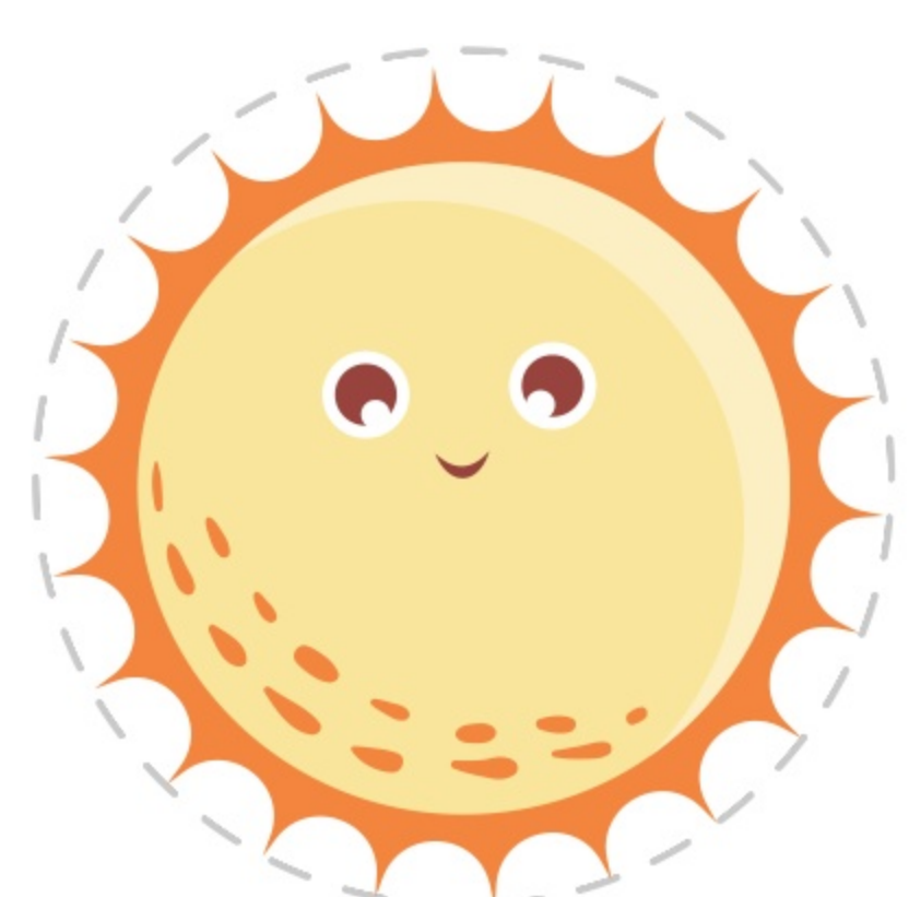
SLUNCE
